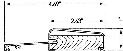
21 OUTSWING THRESHOLD
