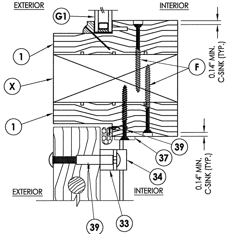
4 VERTICAL CROSS SECTION 4 Outswing
